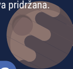
Pluton
